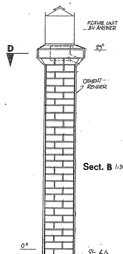
Sect. D 1:10
