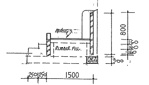
Sect. C
